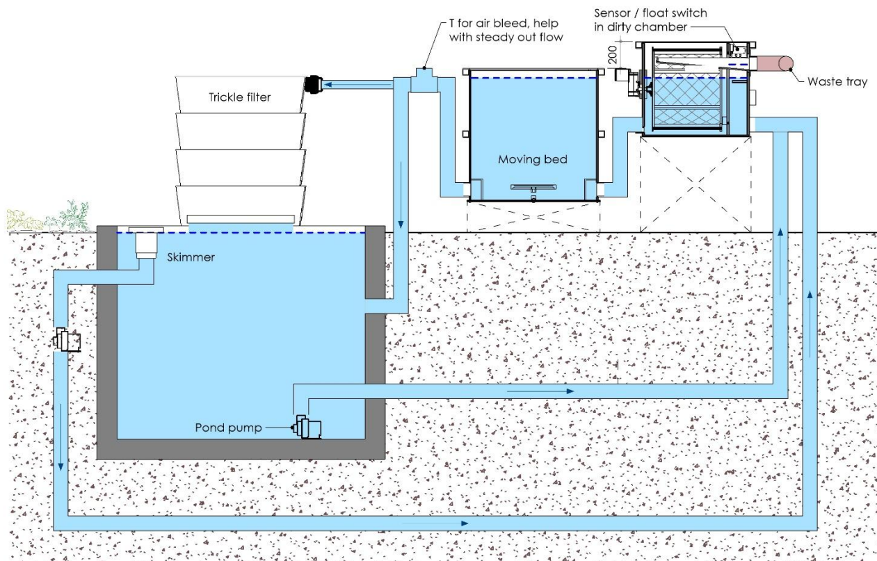
Pic. 4.1 Schematic setup of the drum filter
