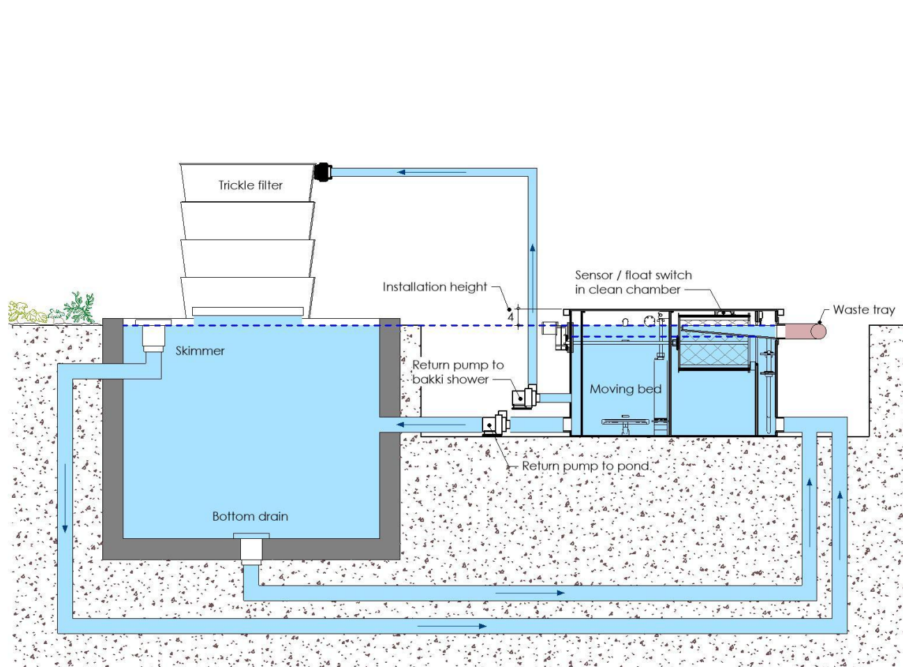
Pic. 3.4 Schematic setup of the combi filter
